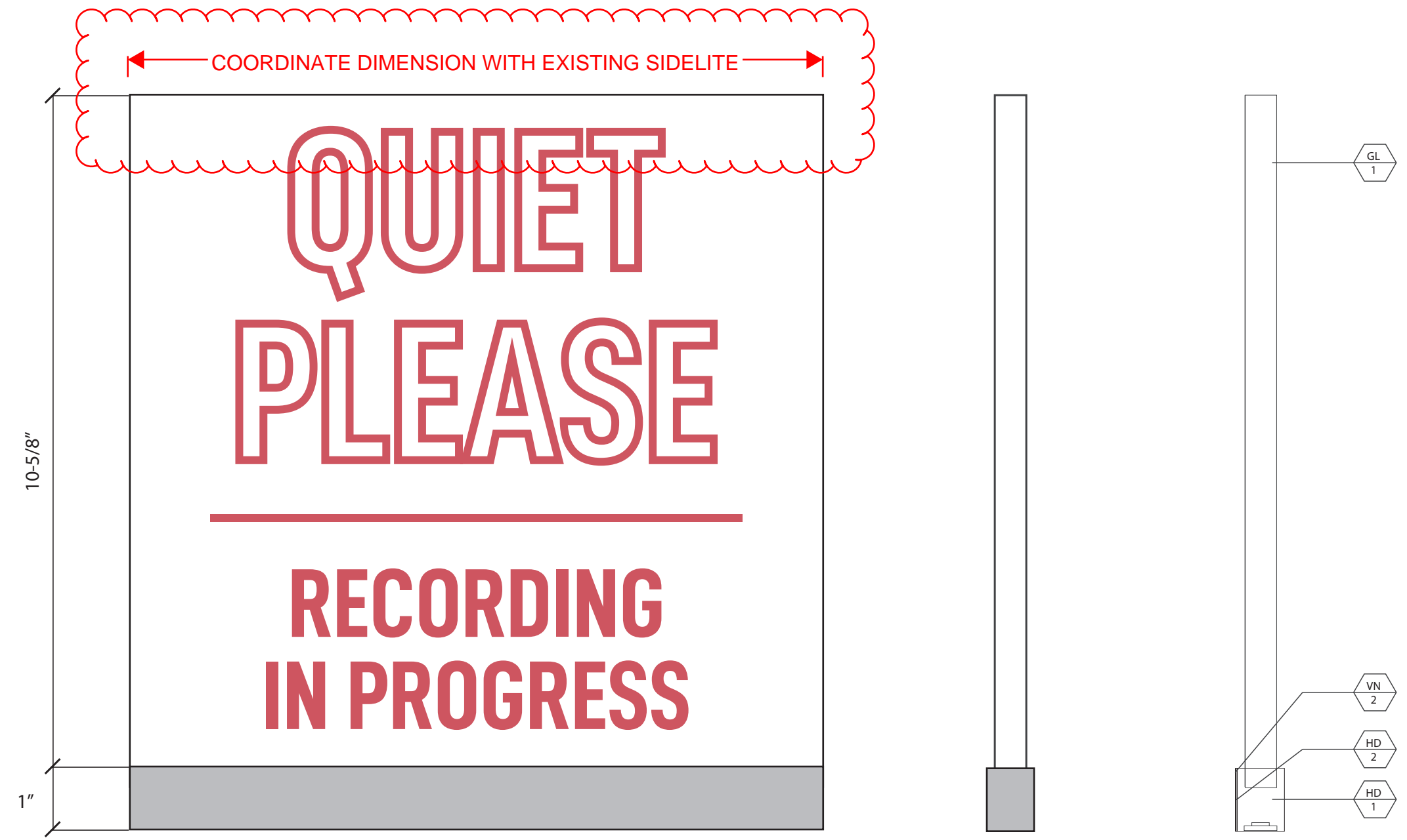
1 ON AIR SIGNAGE DETAILS / SECTION VIEW
