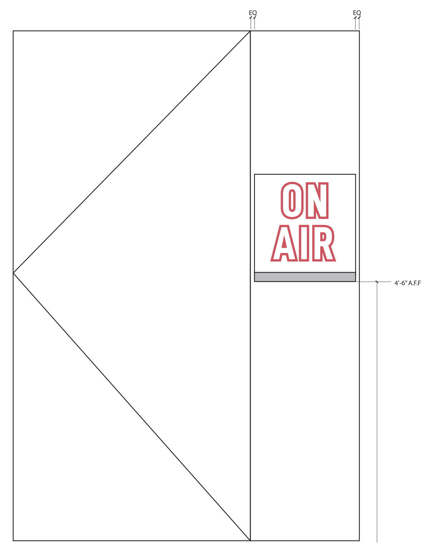
3 ON AIR SIGN MOUNTING ELEVATION
